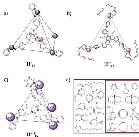
Fig. 6 Representation of tetrahedral cages: (a) \text{II}^{\text{f}}_{\text{Fe}} , (b) \text{II}^{\text{f}}_{\text{Fe}} , (c) \text{II}^{\text{vf}}_{\text{Fe}} and (d) guest molecules encapsulated in cage \text{II}^{\text{vf}}_{\text{Fe}} , in \text{D}_2\text{O} all molecules whereas there is a subset in \text{CD}_3\text{CN} . Reproduced with permission from ref. 51–53. Copyright 2018, John Wiley & Sons, Ltd; 2019, and 2014, the American Chemical Society.
