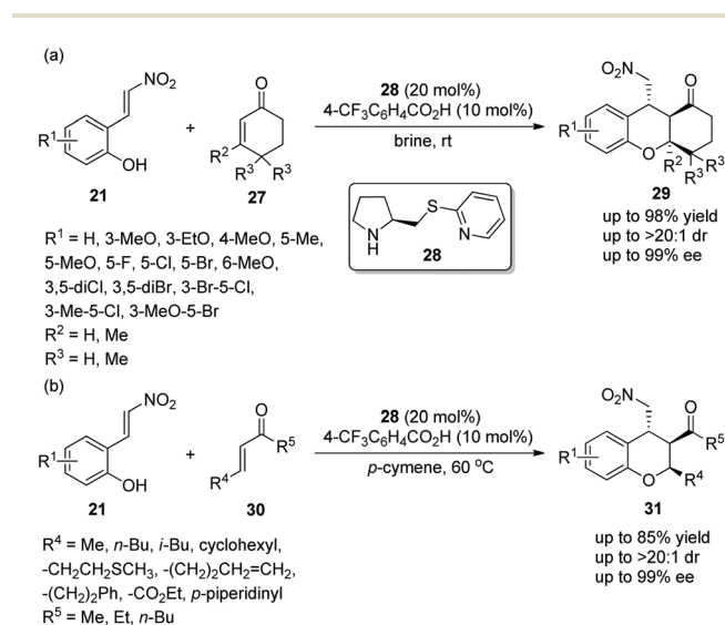
Scheme 9 Oxa-Michael/Michael cascade reaction for the synthesis of tetrahydroxanthenones and chromans.
