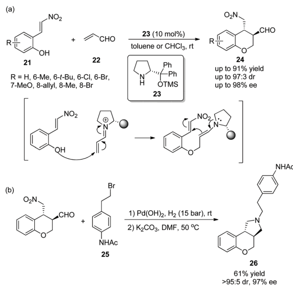
Scheme 8 Oxa-Michael/Michael cascade reaction for the synthesis of 3,4- trans -disubstituted chromans and the derivatization of chiral chroman.
