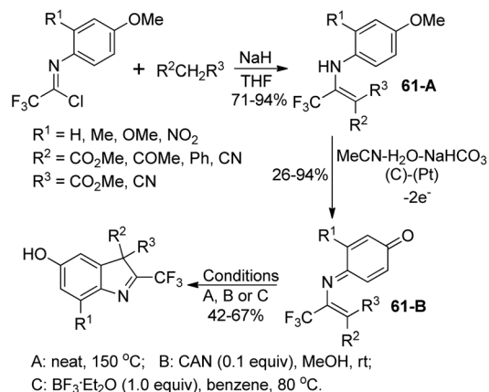
Scheme 61 Synthesis of 2-(trifluoromethyl)-3H-indoles.
