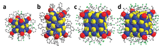
Fig. 5 X-ray structures of Ag cubes: \text{Ag}_{14}(\text{SC}_6\text{H}_3\text{F}_2)_{12}(\text{PPh}_3)_8 , \text{Ag}_{23}(\text{PPh}_3)_8(\text{SC}_2\text{H}_4\text{Ph})_{18} , \text{Ag}_{38}(\text{SPhF}_2)_{26}(\text{P}^t\text{Bu}_3)_8 , and \text{Ag}_{63}(\text{SPhF}_2)_{36}(\text{P}^t\text{Bu}_3)_8 . Adapted with permission from ref. 62. Copyright 2019, Royal Society of Chemistry.
