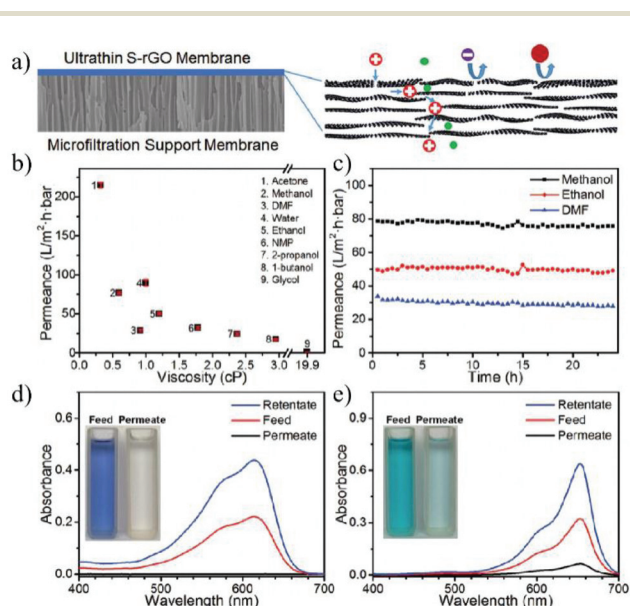
Fig. 19 (a) Schematic illustration of the ultrathin S-rGO membrane coated on the surface of a microporous substrate and the separation mechanism of the S-rGO membrane. (b–e) The nanofiltration performance of S-rGO and HPEI/S-rGO membranes. 177 Copyright, 2016 Wiley-VCH.
