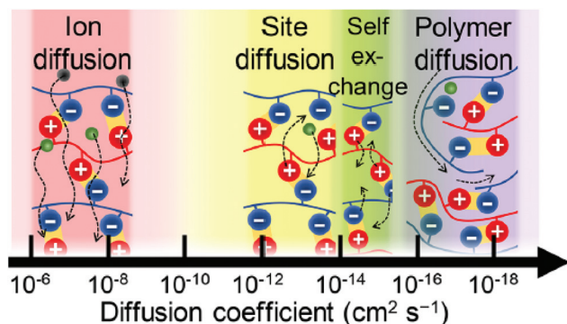
Fig. 5 Intrinsic and extrinsic diffusion processes within ionic polymeric materials ranked according to their diffusion coefficients. Reprinted with permission from ref. 56. Copyright 2017, American Chemical Society.
