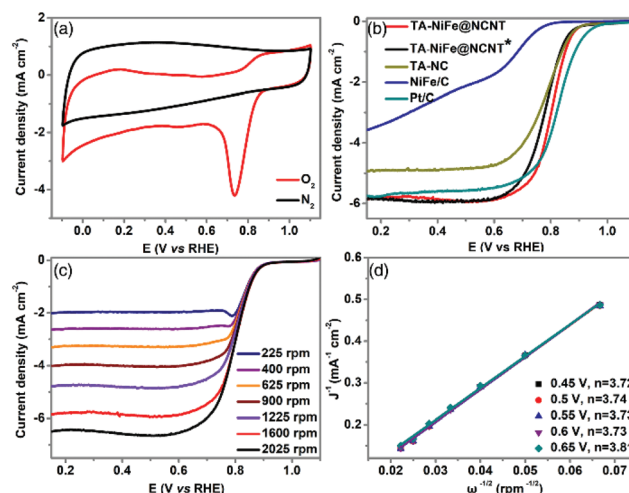
Fig. 4 (a) CV curves for TA-NiFe@NCNT in \text{O}_2 and \text{N}_2 saturated 0.1 \text{ M KOH} electrolytes collected at a scan rate of 100 \text{ mV s}^{-1} . (b) ORR LSV curves for TA-NiFe@NCNT, TA-NiFe@NCNT*, TA-NC, NiFe/C, and Pt/C collected at a rotation speed of 1600 \text{ rpm} and a scan rate of 10 \text{ mV s}^{-1} . (c) ORR LSV curves for TA-NiFe@NCNT at various rotation speeds. (d) K-L plots for TA-NiFe@NCNT at different potentials derived from the corresponding ORR LSV curves.
