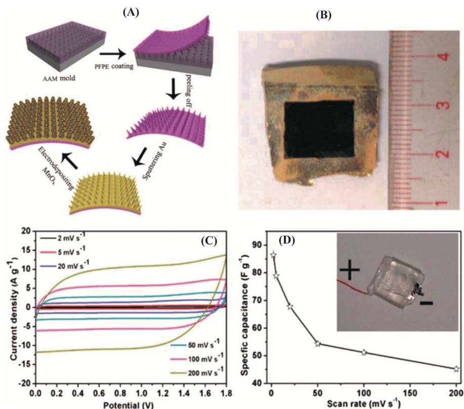
Fig. 1 Fabrication of the 3D metal/oxide nanocone array electrode. (A) Schematic diagram of the fabrication process of the 3D flexible nanocone array electrode. (B) Optical image of an as-prepared 3D Au/MnO x nanocone array electrode. Performance testing of a full SC consisting of the 3D Au/MnO x nanocone array positive electrode and a CCG negative electrode. (C) CV curves of the full SC at various scan rates in 1 M Na 2 SO 4 . (D) Corresponding specific capacitance as a function of scan rates. 64
