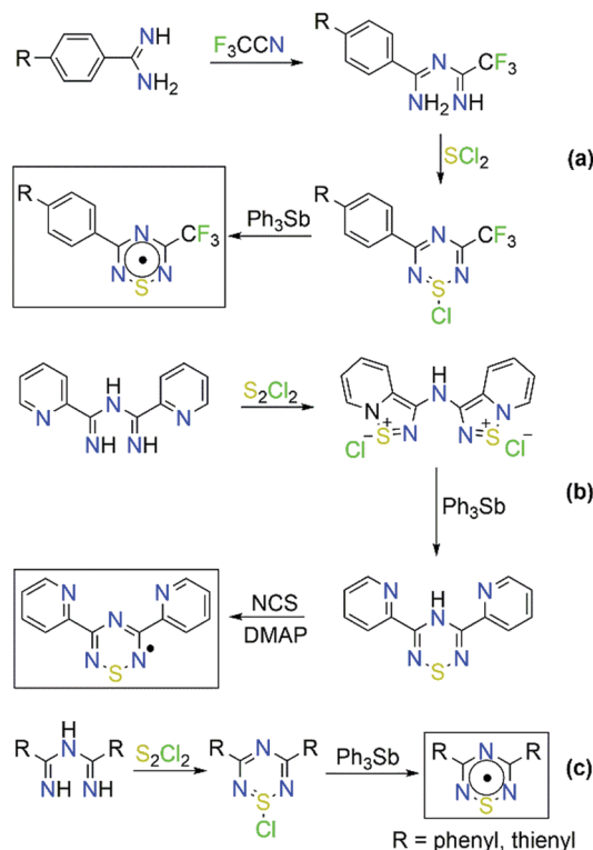
Scheme 7 General synthetic routes for the synthesis of (a) asymmetrical 5-aryl-3-trifluoromethyl-1,2,4,6-thiatiazinyls, (b) symmetrical 3,5-dipyridylthiatiazinyl ( Py 2 TTAH ) and 3,5-bis-(phenyl)-1,2,4,6-thiatiazinyl ( Ph 2 TTA ), and (c) 3,5-bis-(2-thienyl)-1,2,4,6-thiatiazinyl ( Th 2 TTA ). R = phenyl, thienyl
