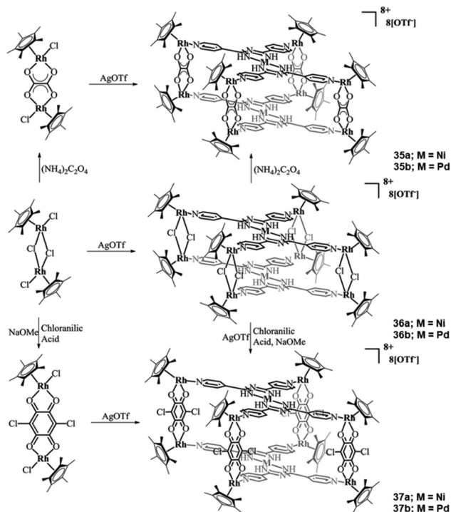
Scheme 14 The synthetic routes that led to the isolation of the organo-metallic heterometallic complexes, where M = \text{Ni}^{\text{II}} or \text{Pd}^{\text{II}} . Adapted with permission from ref. 54. Copyright 2017 Royal Society of Chemistry.
