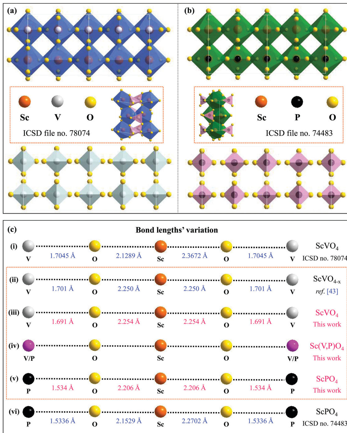
Fig. 1 (a and b) Double cell X [-1 \dots +1] of the \text{ScVO}_4 and \text{ScPO}_4 isostructural crystals based on the ICSD file no. 78074 and no. 74483, respectively, from which we can clearly see the coordination environments of \text{P}^{5+} and \text{Sc}^{3+} cations and that the [\text{ScO}_6] and [\text{PO}_4] polyhedral structures share the same oxygen atoms or the same oxygen edges; (c) The Sc–O and V–O bond lengths of \text{ScPO}_4 and \text{ScVO}_4 based on the ICSD file no. 78074 (i) and no. 74483 (vi), as well as the average lengths of Sc–O and V–O bonds achieved from the \text{ScVO}_{4-x} crystal (ii), 43 and the dependence of the average Sc–O and V/P–O bond length variation on the x value in the as-obtained \text{Sc}(\text{P}_x\text{V}_{1-x})\text{O}_4 ( 0.0 \leq x \leq 1 ) solid solutions (iii–v). Noted that the average interatomic Sc–O and V/P–O distances in (ii), (iii) and (v) were calculated using Vesta software and the atomic positions we used for establishing the model were based on the refined XRD atomic positions. Since the Vesta modeling process does not consider other factors such as the XRD pattern backgrounds, scale factors, and peak shapes, the calculated Sc–O and V/P–O distances are a little shorter than that derived from the refined data, but they are all correct and fine results.
