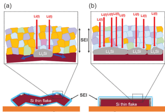
Fig. 8 Schematic illustrations of the SEI film formed during the charge process of the binder-free Si anode in (a) 83.3–16.7 mol% [C_2mim][FSA]-Li[TFSA] and (b) 83.3–16.7 mol% [C_2mim][FSA]-Li[FSA] or 50.0–50.0 mol% [C_2mim][FSA]-Li[FSA] . The parts painted in each color show different components: (blue) LiF; (pink) Li_3N ; (purple) Li_2SO_4 ; (green) Li_2S ; and (orange) sulfone.
