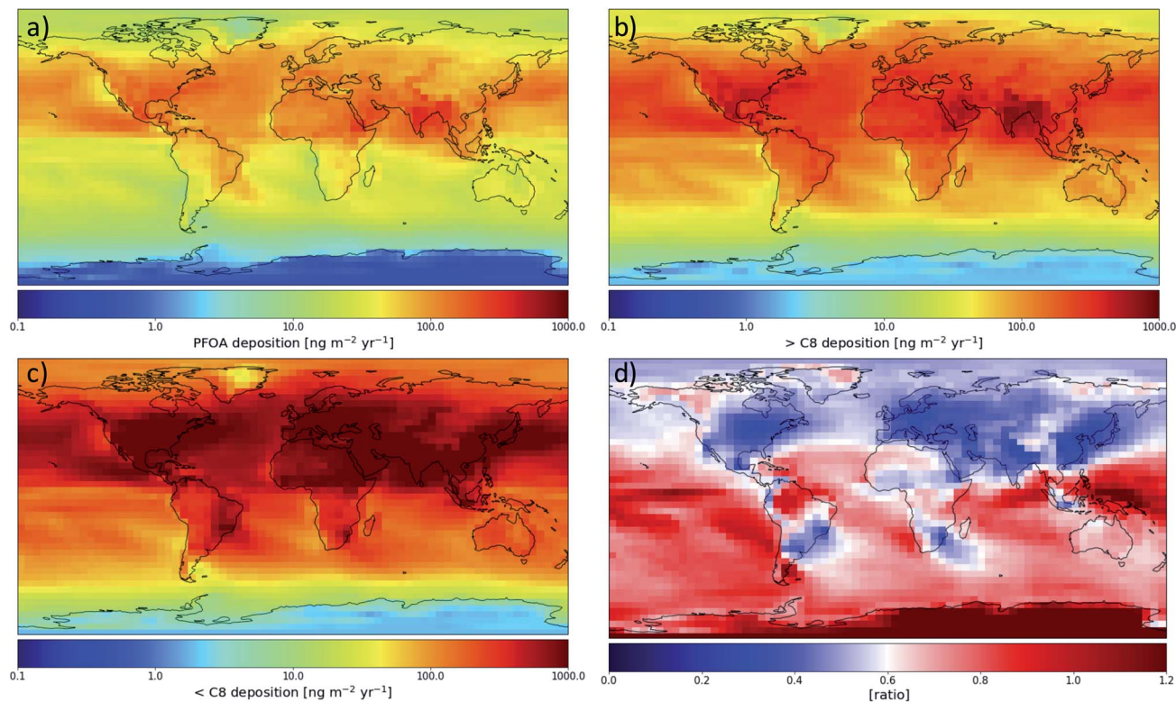
Fig. 2 Spatial distribution of modeled 2013–2015 annual average (a) PFOA deposition ( \text{ng per m}^2 per year), (b) deposition of all longer-chain PFCAs ( \text{ng per m}^2 per year), (c) deposition of all shorter-chain PFCAs, and (d) precursor-produced long-chain (>C7) to short-chain deposition ratio.
