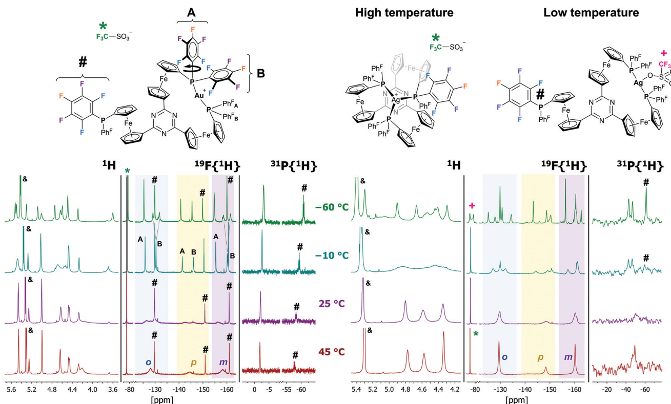
Fig. 5 Sections of the variable-temperature ^1H , ^{19}F\{^1H\} , and ^{31}P\{^1H\} NMR spectra of [1a^F(Au)]OTf (left) and [1a^F(Ag)]OTf (right) in CD_2Cl_2 (&: CHDCl_2/CH_2Cl_2 resonance; *: triflate anion resonance; +: split triflate anion resonance of [1a^F(Ag)]OTf ; #: pendant P(Ph^F)_2 group). The shaded areas in the ^{19}F\{^1H\} NMR spectra correspond to the spectral regions of the ortho (blue), para (orange), and meta fluorine substituents of the P(Ph^F)_2 groups.
