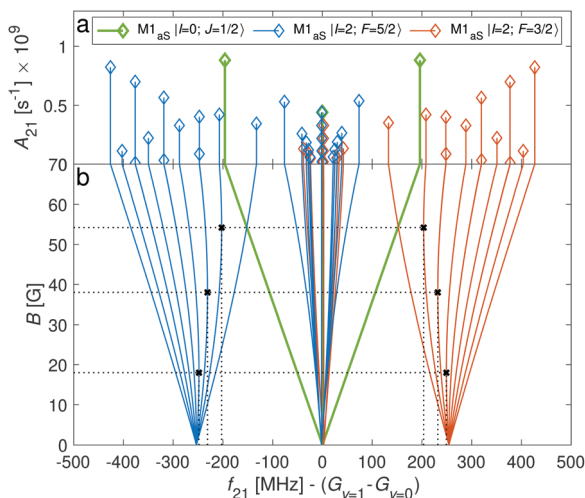
Fig. 11 (a) Einstein A coefficients (b) and line positions as function of magnetic-field strength, B , of hyperfine-Zeeman components of the Q(0) line of the fundamental vibrational transition |v = 0, N = 0\rangle \rightarrow |v' = 1, N' = 0\rangle . Black crosses and dotted lines indicate positions of “magic” magnetic-field transitions.
