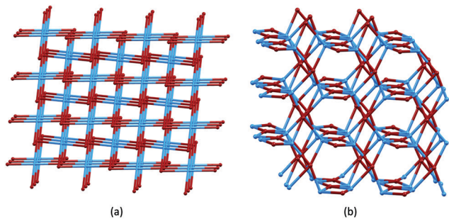
Fig. 7 (a) The cds net found in [\text{Co}(\text{NCS})_2(\mathbf{2})_2]_n , [\text{Co}(\text{NCS})_2(\mathbf{3})_2]_n and [\text{Co}(\text{NCS})_2(\mathbf{11})_2]_n . (b) The lvt net found in [\text{Co}(\text{NCS})_2(\mathbf{8})_2]_n , with ligand nodes in blue and Co nodes in maroon. Both diagrams are TOPOS 49 representations.
