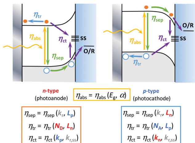
Fig. 2 Scheme with the band structure and the semiconductor electro-lyte interface (SEI) depicting the efficiencies ( \eta ) for all the light-induced processes as a function of different physical magnitudes, in the case of an n-type photoanode (left) and a p-type photocathode (right). Symbols: \eta_{\text{abs}} (yellow), \eta_{\text{sep}} (green), \eta_{\text{tr}} (blue) and \eta_{\text{ct}} (purple) refer to the efficiencies of light absorption, charge separation, majority charge carrier transport, and minority charge carrier transfer processes, respectively; E_g , band gap energy; \alpha , light absorption coefficient; ss, surface states; O/R, dissolved or adsorbed redox couple at the SEI; k_n and k_p , minority carrier transfer rate constants for electrons and holes at the SEI, respectively; k_r and k_{r,ss} , charge recombination rate constants in the bulk and at surface states, respectively; L_n and L_p , diffusion lengths of electrons (majority carriers in photoanodes, minority carriers in photocathodes) and holes (majority carriers in photocathodes, minority carriers in photoanodes), respectively; N_D and N_A , charge donor or acceptor densities in n- or p-type semiconductors, respectively.
