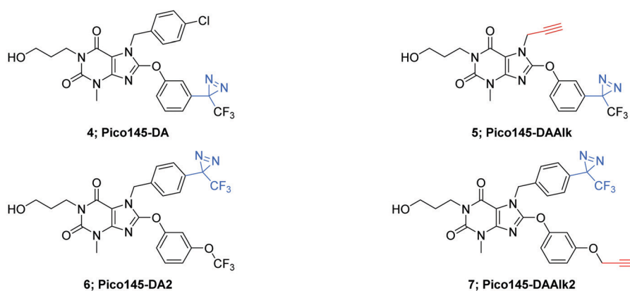
Fig. 1 Structures of xanthine derivatives discussed in this work. (A) Structures of previously described xanthine-based TRPC1/4/5 modulators Pico145 (HC-608) 1 , HC-070 2 and AM237 3 . (B) Structures of new xanthine-based photoaffinity probes described in this work: Pico145-DA 4 (Pico145-diazirine), Pico145-DAAIk 5 (Pico145-diazirine-alkyne), Pico145-DA2 6 (Pico145-diazirine-2) and Pico145-DAAIk2 7 (Pico145-diazirine-alkyne-2). Changes to the Pico145 structure are highlighted in blue (diazirine photocrosslinkers) and red (alkyne handles).
