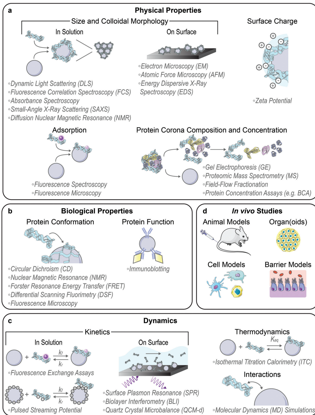
Fig. 2 Modes of characterizing protein–nanoparticle complex formation and performance. (a) Physical properties include complex size and colloidal morphology (preferably characterized in solution over on surface), surface charge, corona adsorption, and corona composition and amount. (b) Biological properties include surface-adsorbed protein conformation and function. (c) Dynamics include kinetics (preferably characterized in solution over on surface), thermodynamics, and interactions. (d) In vivo function can be assessed in model organisms, organs or organoids, cells, and cellular barriers. Some images in this figure are adapted with permission from Servier Medical Art by Servier ( http://smart.servier.com ), licensed under a Creative Commons Attribution 3.0 Unported License.
