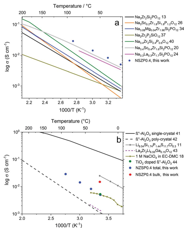
Fig. 4 Temperature dependence of \sigma_{\text{total}} for NZSP0.4 and comparison with (a) other NASICON materials and (b) other Na and Li ion conductors.
