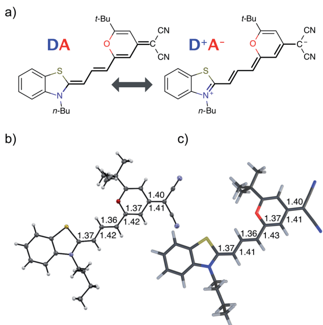
Fig. 1 DCBT structure. (a) Neutral [DA] and zwitterionic [D + A - ] resonance structures of merocyanine dye DCBT . The polymethine chain connecting donor D and acceptor A is highlighted. (b) Molecular structure obtained from crystallographic analysis (thermal ellipsoids are set at 50% probability) (c) DFT calculations using IEFPCM solvation (in DMSO). The bond distances (in Å) along the polymethine chain are shown next to each bond.
