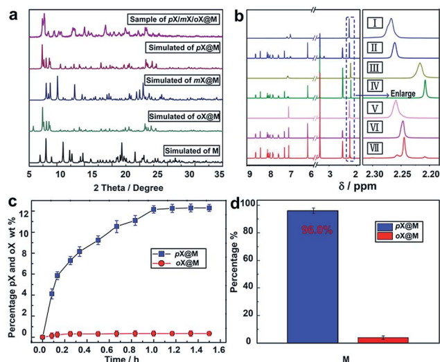
Fig. 3 Separation performance of M towards xylenes. (a) The PXRD pattern of pX/mX/oX@M vs. the calculated PXRD patterns of oX@M , mX@M , pX@M . (b) The ^1\text{H} NMR spectra (DMSO) of M after soaking in xylenes vs. reference extractions. pX is the predominant isomer: (I) mX ; (II) mX@M ; (III) oX ; (IV) oX@M ; (V) pX ; (VI) pX@M ; (VII) xylenes@ M . (c) Kinetics of sorption for pX/oX at 383 K as determined by GC. (d) Relative amount of pX and oX extracted by M as measured by GC (average value of five extractions).
