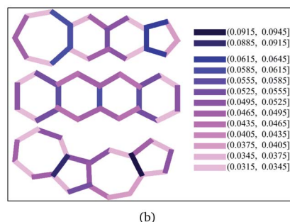
Fig. 4 (a) Example configurations of spins on the polyazulene and fused acene–azulene systems. (b) Probabilities of same spins across bonds.
