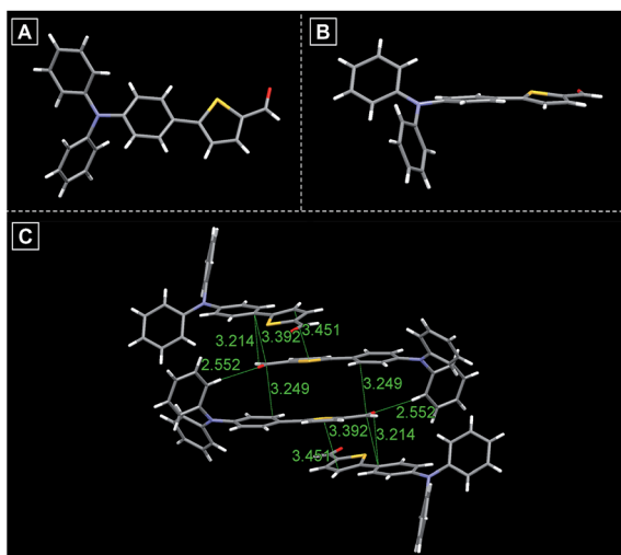
Fig. 2 (A) Single crystal structure of TTV. (B) Side view of the crystal structure of TTV. (C) Various inter- and intramolecular interactions in crystals of TTV.
