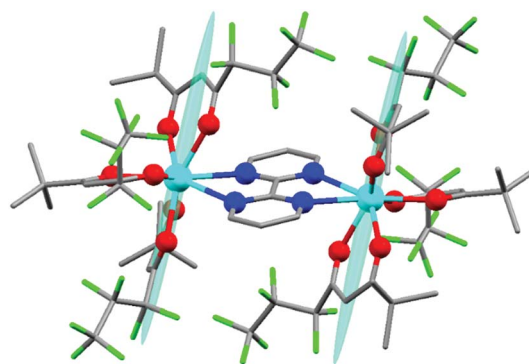
Fig. 1 Chemical structure of the Dy 2 derivative. Colour code: Dy-pale blue, O-red, N-blue, F-green, C-grey. H atoms were omitted for clarity. The pale blue ellipsoids are the susceptibility tensors ( \chi ) experimentally obtained with torque magnetometry. The smallest ( x and y ) components of the tensor were magnified by a factor 10 for clarity reasons.
