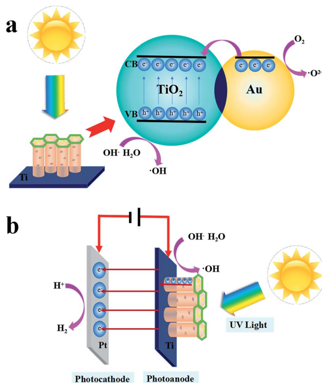
Scheme 2 (a) PC mechanism of the Au/TiO 2 NTs; (b) PEC mechanism of the Au/TiO 2 NTs.
