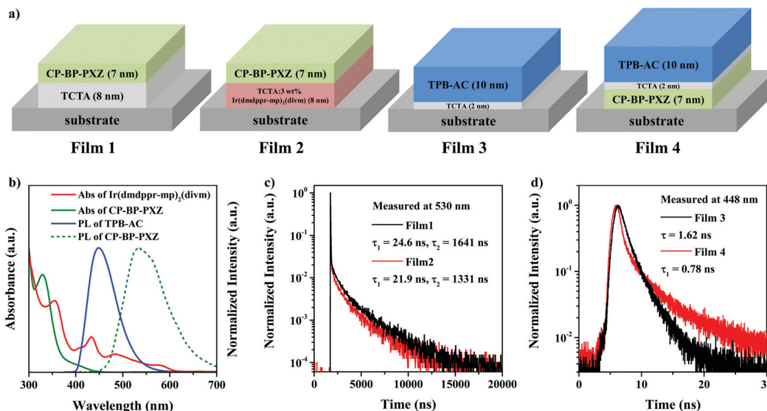
Fig. 4 (a) Structures of films 1–4. (b) Absorption spectra of the Ir(dmprr-mp) 2 (divm) and CP-BP-PXZ films, and PL spectra of the CP-BP-PXZ and TPB-AC films. (c) Transient PL spectra of films 1 and 2 measured at 530 nm. (d) Transient PL spectra of films 3 and 4 measured at 448 nm.
