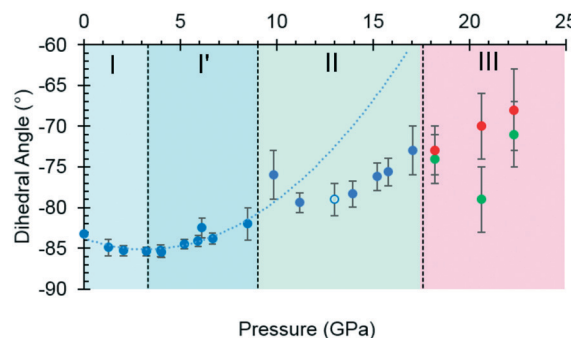
Fig. 4 The O2–C1–C2–C3 torsion angle ( \tau ) as a function of pressure. The green and red circles in phase III represent molecules A and B, and the open circle represents the decompression measurement. A second order polynomial was fitted to phase I and I' data, the minimum of the parabolic function was determined to be -85.0^\circ at 3.3 GPa. Extrapolating the curve to 17.1 GPa serves to highlight the slower rate of change exhibited in phase II. Plots of other torsion angles against pressure are available in the ESI†.
