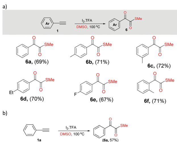
Scheme 4 Studies related to 2-oxomethylthioesters. (a) Substrate scope. Reaction condition: arylacetylene 1 (1.0 mmol), I 2 (2.2 mmol), TFA (1.0 mmol) in 3 mL of DMSO at 100 °C for 4 h. (b) Gram scale synthesis of S-methyl-2-oxo-2-phenylethanethioate. Reaction condition: arylacetylene 1 (9.8 mmol), I 2 (21.6 mmol), TFA (9.8 mmol) in 30 mL of DMSO at 100 °C for 8 h.
