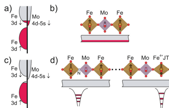
Fig. 1 (a) Schematic band filling of Sr 2 FeMoO 6 . The Fermi level is nearby the bottom of Fe-3d g ↓–Mo-(4d,5s)↓ bands. (b) In the oxide FeO 6 and MoO 6 octahedra are regular (top sketch) and the free carriers in the conduction band (bottom sketch) promote long range ferromagnetic order. (c) Schematic band filling of Sr 2 FeMoO 4.9 N 1.1 . The oxidation of cations induced by N reduces the total number of electrons, and the filling of the bands. In the nitridated sample, the Fermi level shifts down to the top of the Fe-3d↑ band. (d) Localized states formed around defect-related potential wells (e.g.: nitride sites, Jahn–Teller Fe 4+ ions) that trap electrons, hindering carrier mobility, weakening double exchange ferromagnetic interactions and cancelling long range ordering.
