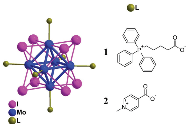
Fig. 1 Schematic representation of the molecular structures of 1 and 2 . Color coding: Molybdenum (blue), iodine (magenta), caboxylated ligands (green), and hydrogen atoms are omitted for clarity.
