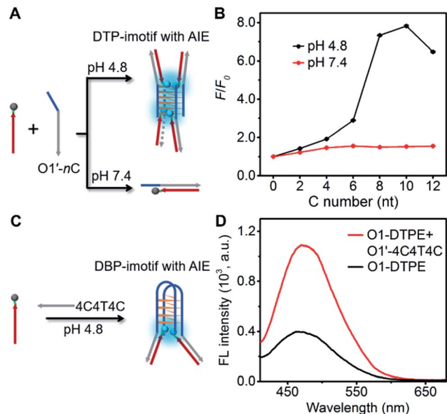
Fig. 6 (A) Schematic illustration of the DTP-imotif structure adopted at pH 4.8 and the double-stranded structure formed at pH 7.4. (B) Ratios of fluorescent peak intensity of 1.0 \mu M O1-DTPE after and before ( F/F_0 ) hybridization with O1'- n C ( n = 0 to 12) in pH 4.8 TAE reaction buffer and in pH 7.4 TE reaction buffer at 25 ^{\circ} C. (C) Schematic illustration of the DBP-imotif structure. (D) Fluorescence spectra of 1.0 \mu M O1-DTPE and the mixture of 1.0 \mu M O1-DTPE and O1'-4C4T4C in pH 4.8 TAE reaction buffer at 25 ^{\circ} C.
