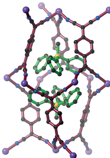
Fig. 12 The structure of (\text{MePPh}_3)_2[\text{M}_1^2(\text{TCNQ})_3] ( \text{M}^{\text{II}} = \text{Zn, Ni, Co, Fe} ) (65–68) in which there is a significant twist in the TCNQ 2- ligands. Pairs of MePPh 3 + cations (green) occupy the intra-framework cavities.
