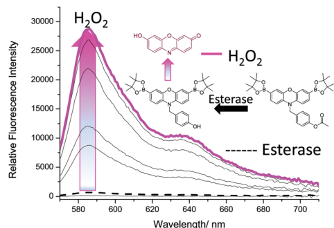
Fig. 5 Fluorescence spectra of Pinkment-OAc (0.5 \mu\text{M} ) for the incubation (15 min) of porcine liver esterase, PLE (0.6 U) followed by incremental additions of \text{H}_2\text{O}_2 (0–1 mM) measurements were taken after 1 h. The data was collected in PBS (100% w/w \text{H}_2\text{O} ) at pH = 7.4, 25 ^\circ\text{C} . \lambda_{\text{ex}} = 545–20 nm. Dashed line represents esterase (0.6 U) addition only.
