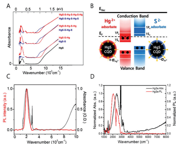
Fig. 4 (A) Absorption spectra of HgS QCD with S^{2-} and Hg^{2+} layer by layer growth. Reprinted with permission from ref. 36 copyright 2014 American Chemical Society. (B) Surface treatment schematics of HgS QCD (C) HgS absorption and photoluminescence spectra reprinted with permission from ref. 39. Copyright 2014 American Chemical Society. (D) HgSe absorption and photoluminescence.
