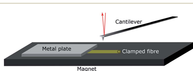
Fig. 1 Custom-made sample holder to clamp fibres onto a hard surface in the AFM liquid cell. The fibres were clamped between a magnet glued into the liquid cell of the AFM and a metal slab with a thickness of 20 \mu\text{m} .
