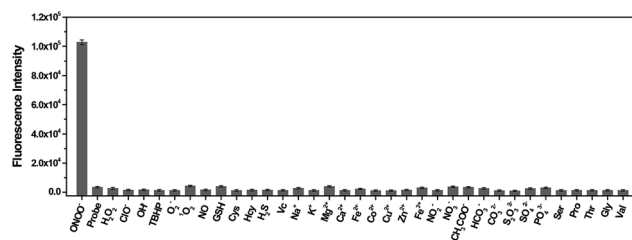
Fig. 1 Fluorescence response of TP-KA (1.0 \mu\text{M} ) with various bio-analytes, including ONOO - (10.0 \mu\text{M} ), H 2 O 2 (200 \mu\text{M} ), other ROS and RNS (10.0 \mu\text{M} ), GSH and Cys (5.0 mM), and other interfering substances (100 mM). The data were recorded after the incubation of TP-KA with various bio-analytes for 10 min at 37 ^{\circ}\text{C} in PBS buffer (50 mM, 7.4) with 1% DMSO. The values are the mean \pm s.d. for n = 3 . \lambda_{\text{ex}}/\lambda_{\text{em}} = 430/560 nm.
