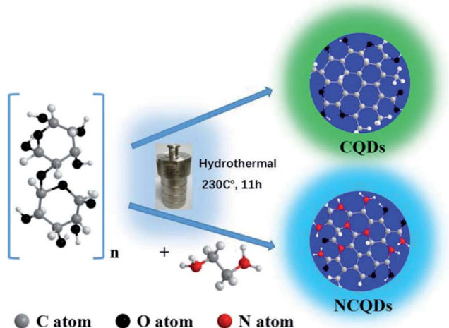
Fig. 1 The synthesis illustration of CQDs and NCQDs.
