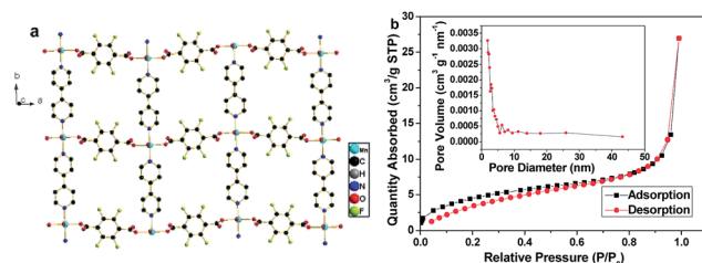
Fig. 4 (a) 2D view of Mn-LMOF. (b) \text{N}_2 adsorption–desorption isotherm of as-synthesized Mn-LMOF after grinding for 2 h, and the inset represents the pore size distribution curve.
