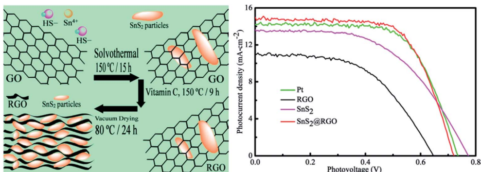
Fig. 18 (Left) illustration depicting preparation of tin sulfide nanoparticles/reduced graphene oxide (SnS 2 @RGO) nanocomposites. (Right) photocurrent density–photovoltage ( J – V ) curves for DSSCs having Pt, RGO, SnS 2 , and SnS 2 @RGO composite CEs. Reprinted with permission from ref. 250, B. Yang, X. Zuo, P. Chen, L. Zhou, X. Yang, H. Zhang, G. Li, M. Wu, Y. Ma, S. Jin and X. Chen, nanocomposite of tin sulfide nanoparticles with reduced graphene oxide in high-efficiency dye-sensitized solar cells. ACS Appl. Mater. Interfaces , 2015, 7, 137–143. Copyright© American Chemical Society.
