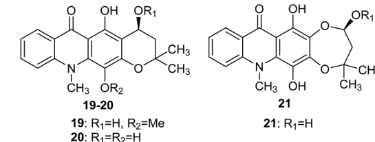
Fig. 4 Structures of acridones (12–21). 36
