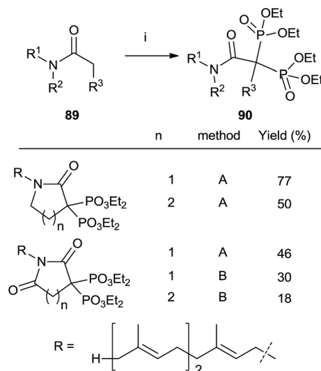
Scheme 23 Reagents and conditions: (i) method A: LDA (2.2 equiv.); then \text{ClP}(\text{OEt})_2 (2.3 eq.); then \text{H}_2\text{O}_2 (10 eq.). Method B: LHMDS; then \text{ClP}(\text{OEt})_2 ; then LHMDS; then \text{ClP}(\text{OEt})_2 ; then \text{H}_2\text{O}_2 (20 eq.).
