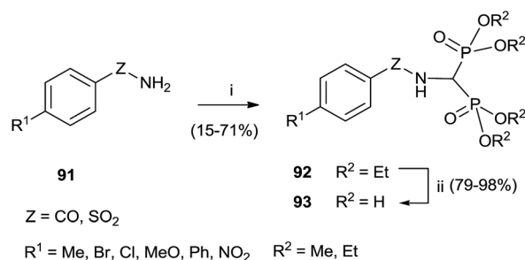
Scheme 24 Reagents and conditions: (i) \text{HC(OR)}_3 , \text{HP(OR)}_2 , 150\text{ }^\circ\text{C} . (ii) \text{BBr}_3 , toluene, MeOH, reflux.
