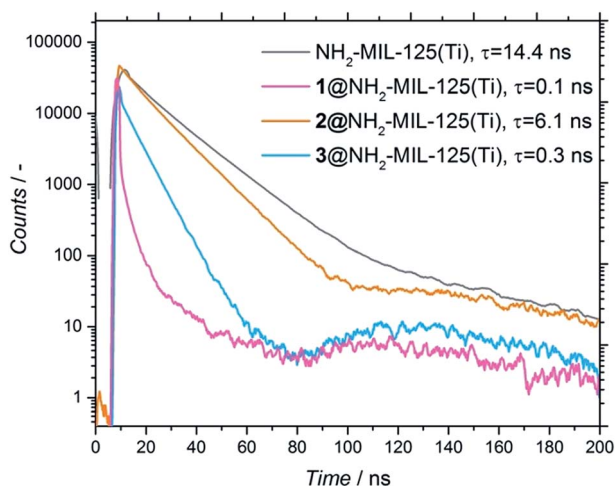
Fig. 5 Time resolved fluorescence of \text{NH}_2\text{-MIL-125(Ti)} in water (grey), 1@\text{NH}_2\text{-MIL-125(Ti)} in acetonitrile (pink), 2@\text{NH}_2\text{-MIL-125(Ti)} in DMF (orange) and 3@\text{NH}_2\text{-MIL-125(Ti)} in water (blue). The suspensions were excited by a 404 nm laser. The decrease in fluorescence over time was measured at a wavelength of 430 nm and fitted by a sum of exponential decays (only the fastest \tau component, which is the biggest contribution, is shown for clarity).
