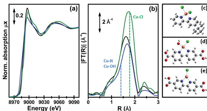
Fig. 8 Part (a): Cu K-edge XANES spectra of the \text{tBpyCuCl}_2 model compound (green) and of the UiO-67-Cu MOF before and after the in situ thermal activation in an \text{N}_2 flow (black and blue spectra, respectively). Part (b): as part (a) for the k^3 -weighted, phase uncorrected FT of the corresponding EXAFS data. Also highlighted with blue and green dashed lines are the typical positions of the (Cu–N or Cu–OH) and Cu–Cl contributions, respectively. Part (c): structure of the \text{tBpyCuCl}_2 model compound as obtained from the single-crystal XRD refinement (data collected at 100 K). Parts (d) and (e): DFT-optimized structures of the \text{Cu(II)ClOH(H}_2\text{bpydc)} and \text{Cu(I)Cl(H}_2\text{bpydc)} complexes used as a starting point for the EXAFS fits of the UiO-67-Cu MOF before and after the in situ thermal activation. Atom colour code: Cu: orange; O: red; N: blue; Cl: green; C: gray; H: white. Previously unpublished figure reporting spectra and structures from ref. 60.
