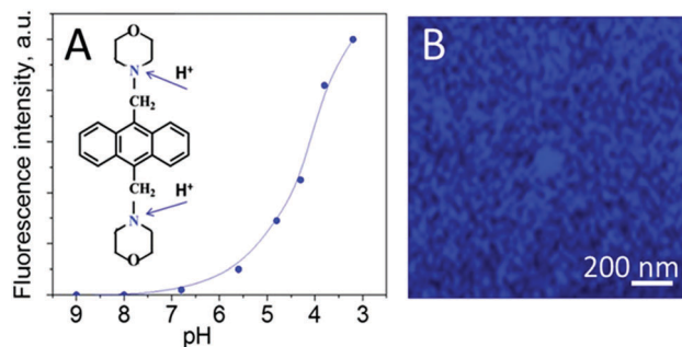
Fig. 3 (A) Calibration of fluorescent pH indicator, 4,4'-(anthracene-9,10-diyl)dimethanediyl)dimorpholine, that exhibits a pK_a \sim 5.1 , and initial chemical formula showing the protonation sites; (B) confocal fluorescent images of the TiO_2 surface immediately after irradiation.
