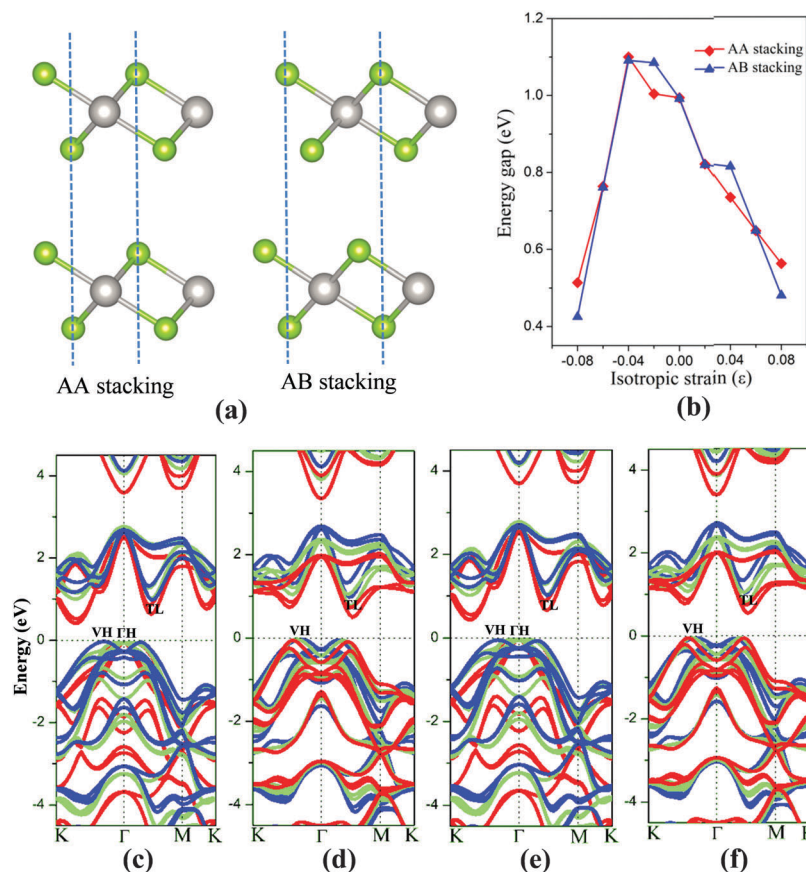
Fig. 5 (a) Atomic structure of two kinds of PtSe 2 bilayers. (b) Band gap of PtSe 2 bilayers versus isotropic strain. Computed band structure of AA stacking bilayers under (c) \epsilon = -8 to 0\% , (d) \epsilon = 0 – 8\% and AB stacking bilayers under (e) \epsilon = -8 to 0\% , (f) \epsilon = 0 – 8\% . The bands with different colors represent the band structures under various strain values, i.e., blue ( \epsilon = 0\% ), green ( \epsilon = \pm 4\% ) and red ( \epsilon = \pm 8\% ). The Fermi level is located at 0 eV.
