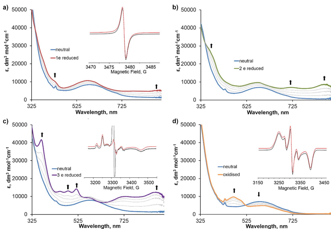
Fig. 2 UV/vis spectra of 3 (blue line in all cases) and the different electrochemically generated radical ion species for the formation of (a) \mathbf{3}^{1-} (red line), (b) \mathbf{3}^{2-} (green line), (c) \mathbf{3}^{3-} (purple line) and (d) \mathbf{3}^{1+} (orange line) with transitional spectra included for all processes (grey lines). All spectra were recorded in DMF solution containing 0.2 M [ ^n\text{Bu}_4\text{N}][\text{BF}_4] as supporting electrolyte. The X-band EPR spectra (black line, inset) and corresponding simulated EPR spectra (red line, inset) of each electrochemically generated species were recorded as (a) a fluid solution spectra for \mathbf{3}^{1-} at 298 K, (c) a frozen solution spectra of \mathbf{3}^{3-} at 77 K, and (d) a frozen solution spectra for \mathbf{3}^{1+} at 77 K.
