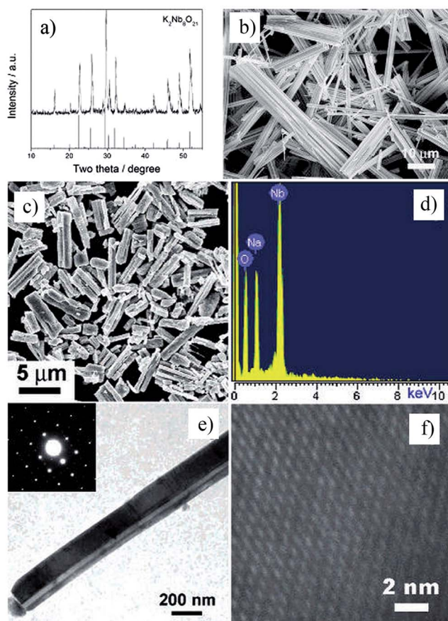
Fig. 2 (a) XRD and (b) SEM images of the potassium niobate nanowires. The angles for the standard sample of potassium niobate are shown in the lower part of panel a. (c) SEM image of sodium niobate nanorods. (d) EDX spectrum showing the complete conversion from K niobate to Na niobate. (e) TEM image of an individual sodium niobate nanorod. Inset is the corresponding SAED pattern. (f) High-resolution TEM image of the same nanorod shown in panel e (ref. 32 Copyright 2007, American Chemical Society).
