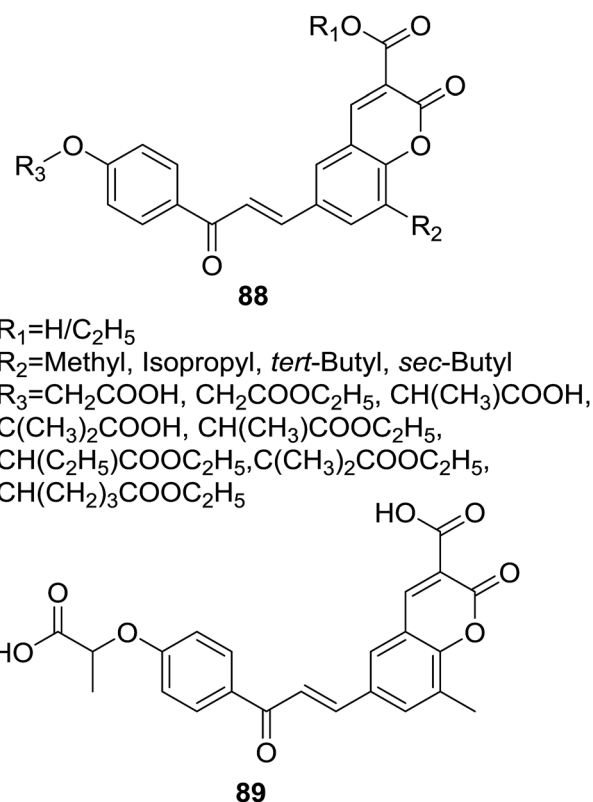
Fig. 25 Coumarin–chalcone hybrid based fibrate like lipid lowering agents.
