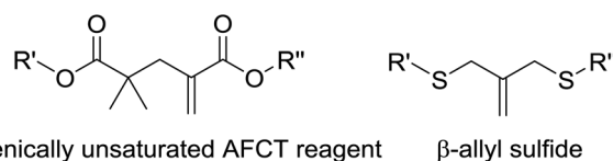
Fig. 19 AFCT reagents used in photopolymerized crosslinked networks.
