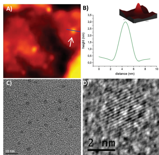
Fig. 5 (A) STM image ( 150 \times 150 \text{ nm}^2 ) showing isolated SiNCs functionalized with n -hexyllithium; (B) STM topographic image of a single SiNC marked by the white arrow in (A) and a cross-section taken along the blue line. (C) TEM image of n -hexyllithium functionalized Si-NCs with an average diameter of 3 nm; (D) HR-TEM image of 3 nm SiNCs functionalized with n -hexyllithium, lattice-fringes are clearly observable. Both methods verify a 3 nm average size of the SiNCs.
